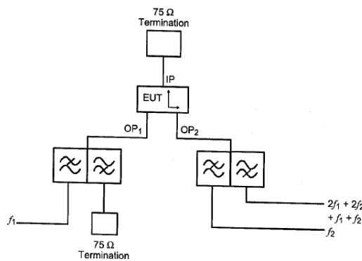
Figure 8 - Harmonic/Intermodulation test circuit
