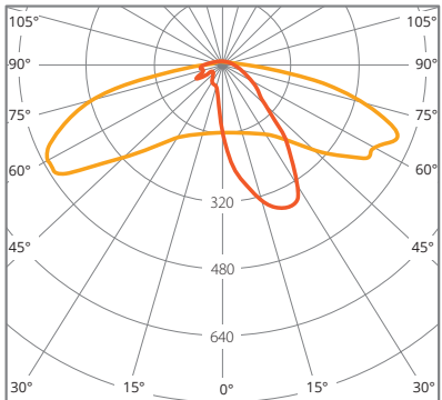
cd/klm ■ C0 - C180 ■ C90 - C270 \eta = 90\%
