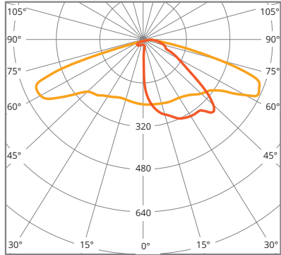
cd/klm ■ C0 - C180 ■ C90 - C270 \eta = 94\%
