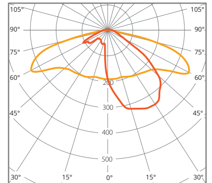
cd/klm ■ C0 - C180 ■ C90 - C270 \eta = 92\%
