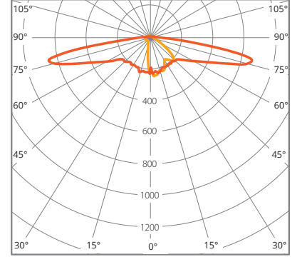
cd/klm ■ C0 - C180 ■ C90 - C270 \eta = 96\%
