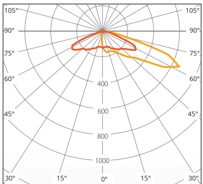
cd/klm ■ C0 - C180 ■ C90 - C270 \eta = 96\%
