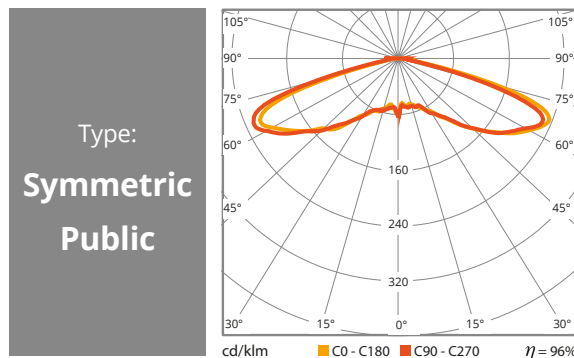
Approximate reference illumination diagrams
