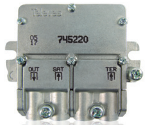
▲ Mini-mixer (745220) 57 x 47 x 13 mm
