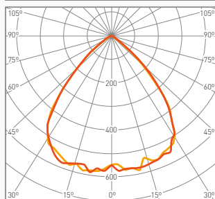
Symmetrical 90° S90
