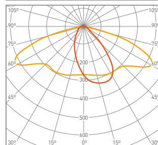
Asymmetric T2C-90
