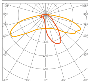
Asymmetric T2
