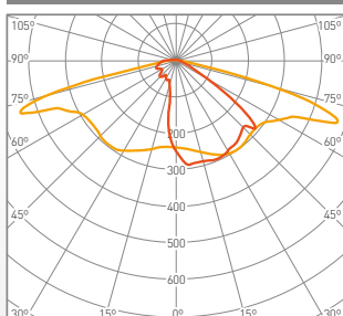
Asymmetric T3B-90
