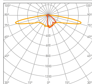
Asymmetric SCL
