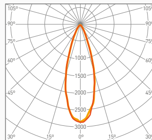
Symmetrical 30° S30
