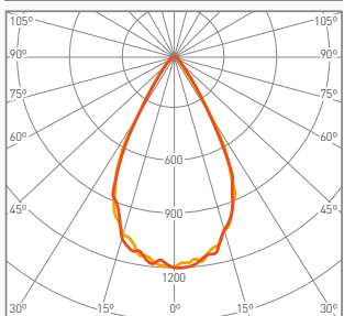
Symmetrical 60° S60
