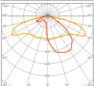
Asymmetric T3
