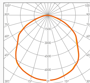
Symmetrical 120° S120
