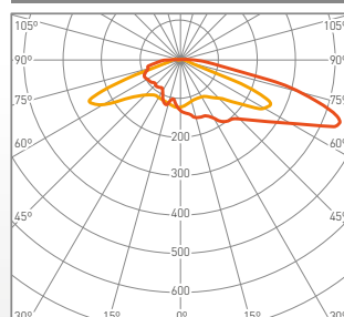
Asymmetric T4
