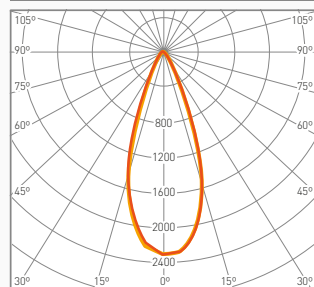
Symmetrical 40° S40
