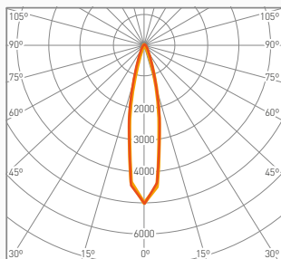
Symmetrical 20° S20
