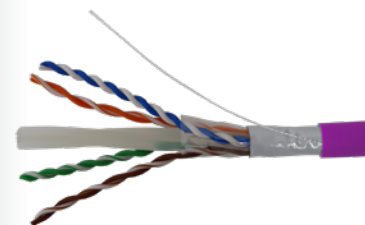
▲ CAT6ALU500V (219312)
